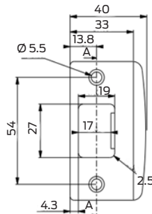
Standard D - Strike Plate
