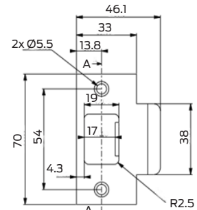
Extended Lipped Strike Plate
